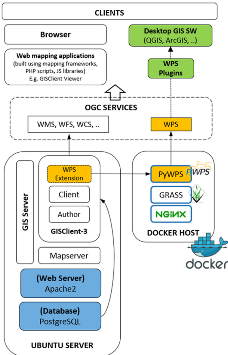
Fig. 6 Project architecture where the PyWPS server is realized using the Docker technology (the container is build up with GRASS GIS support, Gunicorn and Nginx) and a WebGIS Platform is implemented on a Linux Server to test the usability by browser of the web processing services
