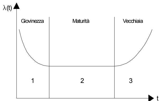
Figura 8 Curva bathtub.
