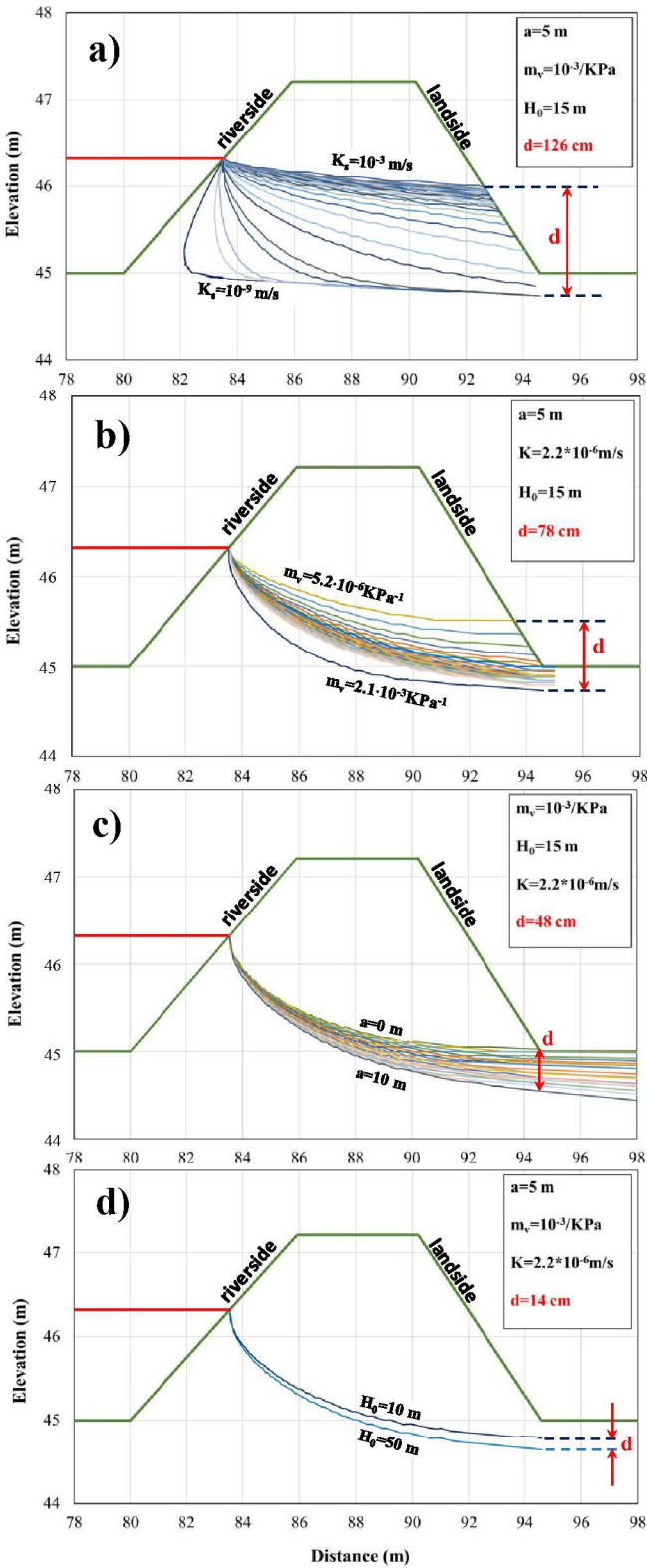
Figure 9: Sensitivity of the seepage line to the geotechnical and geometrical parameters used in SEEP/W simulations: a) soil hydraulic conductivity, K_s ; b) soil volumetric compressibility, m_v ; c) water table depth, a ; d) thickness of the aquifer, H_0 .
