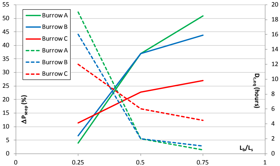
Figure 15: Effect of the burrows for Ta_07_dx levee, in terms of critical equivalent durations, D_{c,eq} reduction (dashed coloured lines) and percentage seepage probability variation, \Delta P_{seep} (%) (solid coloured lines) for different locations and lengths of the cavities.
