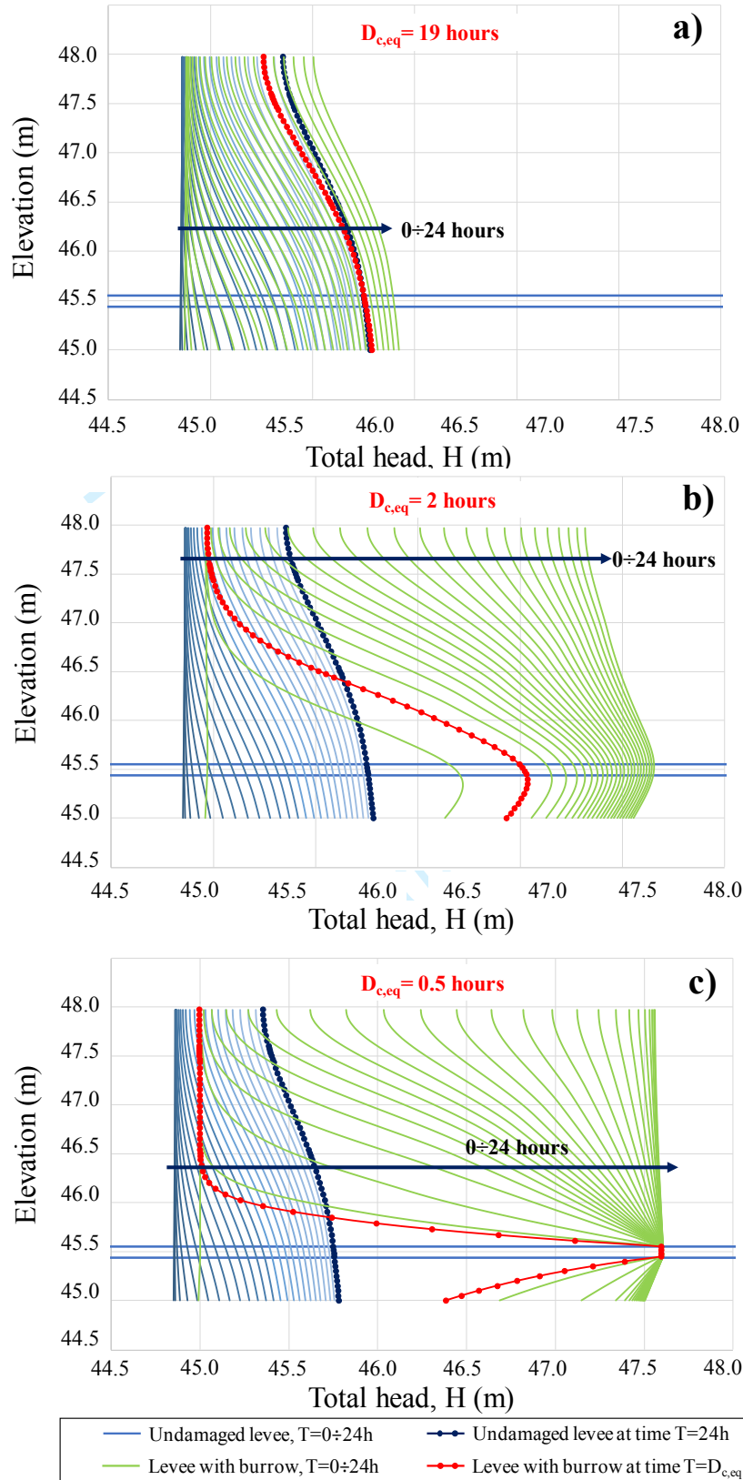
Figure 13: Total heads profiles corresponding to the vertical section crossing the centreline of the levee Ta_07_dx for burrow in A position ( h_b=1/6H_s ) and increasing lengths of the cavity: a) L_b=1/4L_s(h_b) ; b) L_b=1/2 L_s(h_b) ; c) L_b=3/4 L_s(h_b) .
