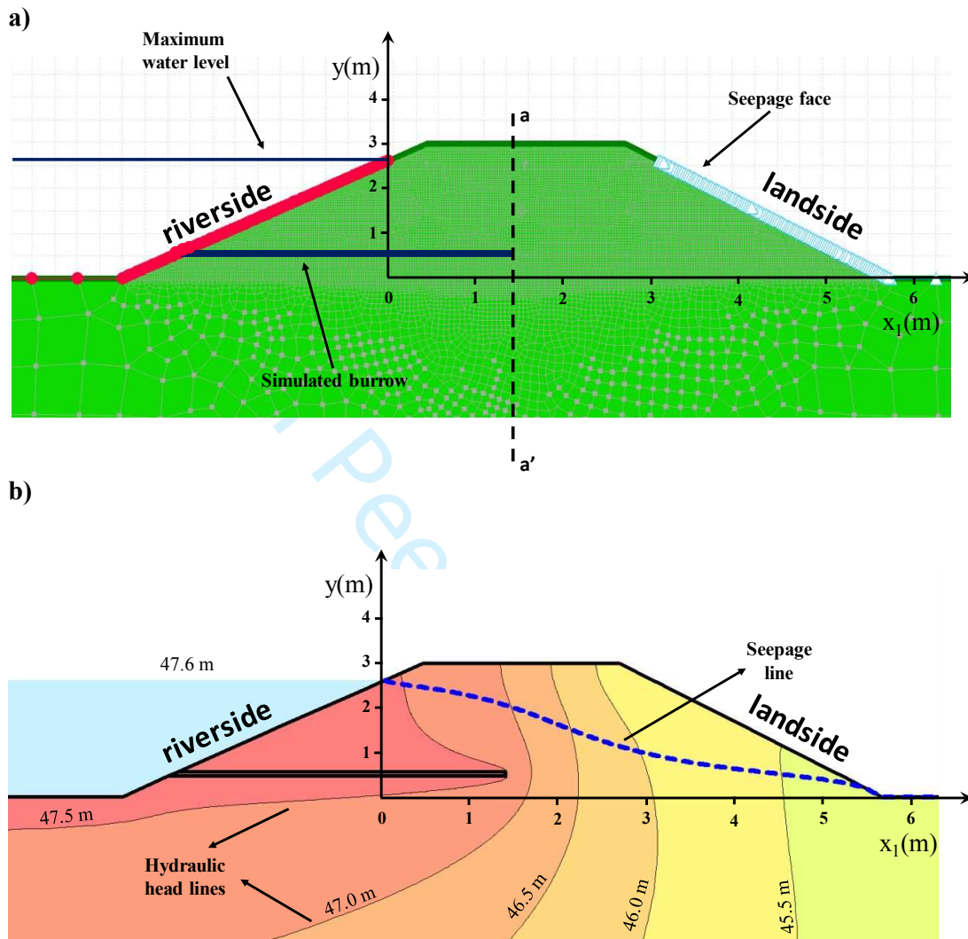
Figure 4: Modelling of the levee affected by burrow in SEEP/W (GEOSTUDIO® 2012 Office): a) sketch of the seepage domain, hypothesised burrow and established boundary conditions for the transient analysis: a rectangular hydrograph with h_0' = H_{200} is simulated in the river channel; \theta_s = 0.51 \text{ m}^3/\text{m}^3 ; \theta_r = 0.102 \text{ m}^3/\text{m}^3 ; m_v = 6 \cdot 10^{-5} \text{ KPa}^{-1} ; the black dashed line identifies the vertical section where the total heads distribution is computed; b) simulation results in terms of hydraulic head contour lines in meter.
