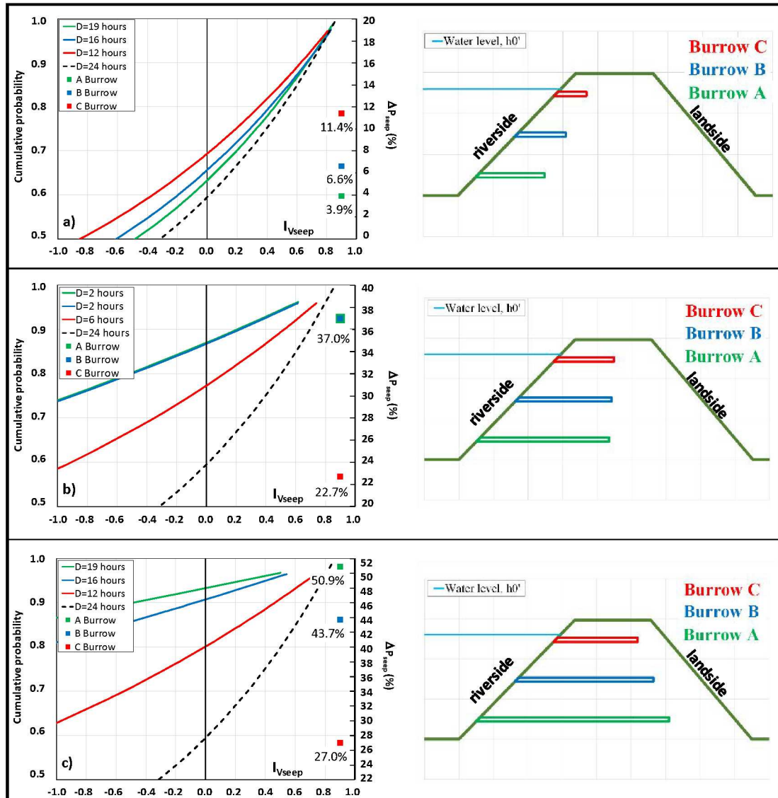
Figure 14: Seepage probability variation induced by the burrows in the Ta 07_dx levee, for different configurations of the cavities: a) burrow (A, B or C) with L_b = 1/4 L_s(h_b) ; b) burrow (A, B or C) with L_b = 1/2 L_s(h_b) ; c) burrow (A, B or C) with L_b = 3/4 L_s(h_b) .
