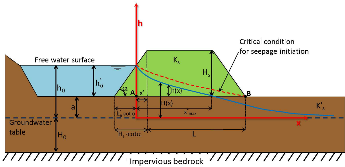
Figure 1: Scheme of earthen levee and representation of the variables adopted for the definition of the seepage line according to Marchi solution (1961). For symbols, see text. Adapted from Barbetta et al. (2017).
