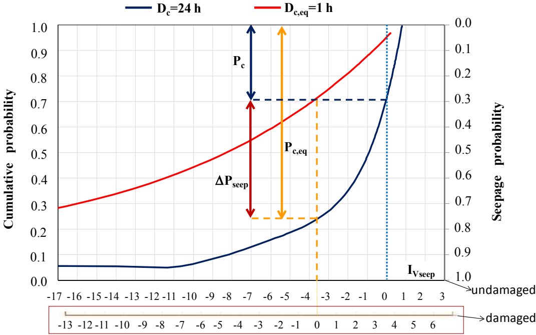
Figure 6: Seepage probability variation induced by the presence of the burrow in the levee, \Delta P_{seep} . The fragility curves refer to an undamaged levee and are estimated by the expeditious procedure (Barbetta et al., 2017). The upper I_{vseep} axis is referred to the undamaged levee, while the lower axis is referred to the damaged one.
