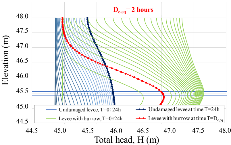
Figure 5: Evolution of the total head profiles across the vertical section crossing the centreline of the levee: 1) light blue lines=total heads in the intact levee, for hourly time steps in the interval 0 \div T=24 hours; 2) green lines=total heads in the levee with burrow, for hourly time steps in the interval 0 \div T=24 hours; 3) dark blue line=total head profile in the undamaged levee, corresponding to a flood duration T=24 hours; 4) red line=total head profile in the damaged embankment, for a flood duration equal to the equivalent critical duration, D_{c,eq}=2 hours.
