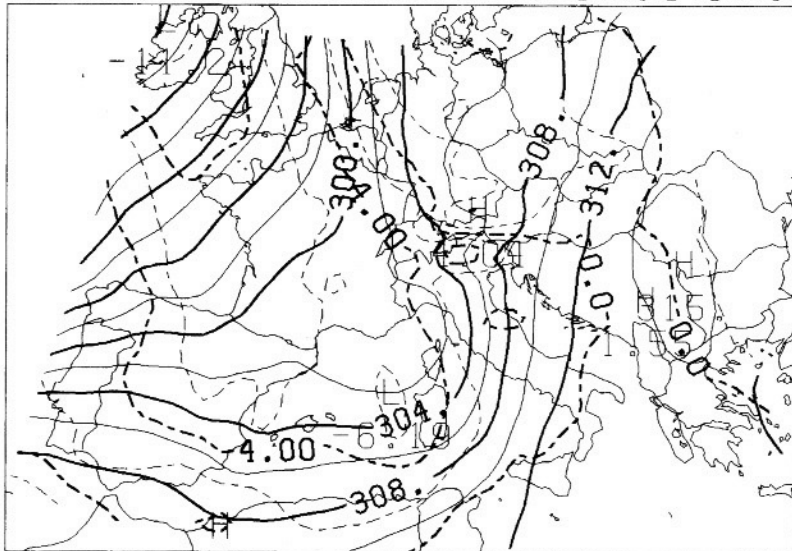
GRIB ANALYSIS AT 06/11/94 06:00 GMT (DOM)
