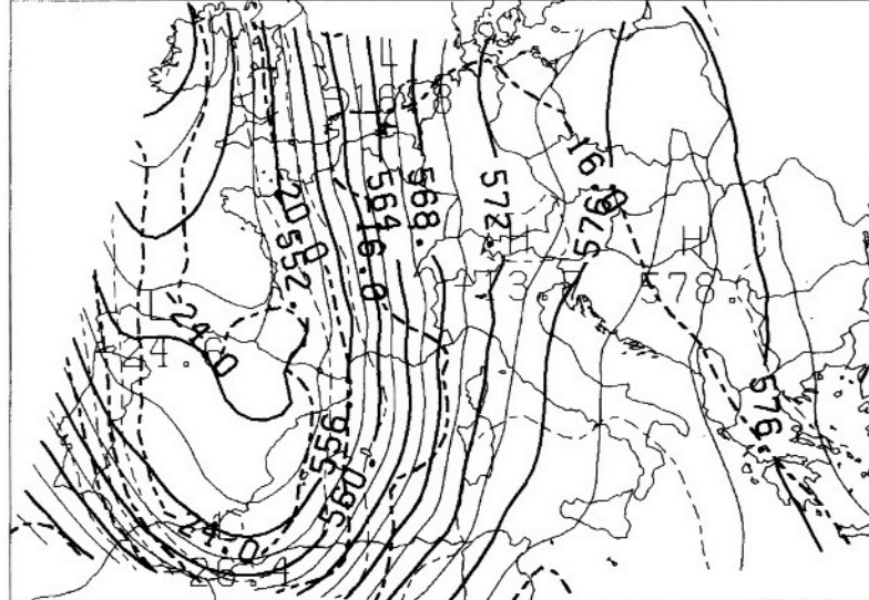
GRIB ANALYSIS AT 05/11/94 12:00 GMT (SAB)
