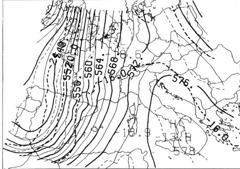
GRIB ANALYSIS AT 04/11/94 12:00 GMT (VEN)
