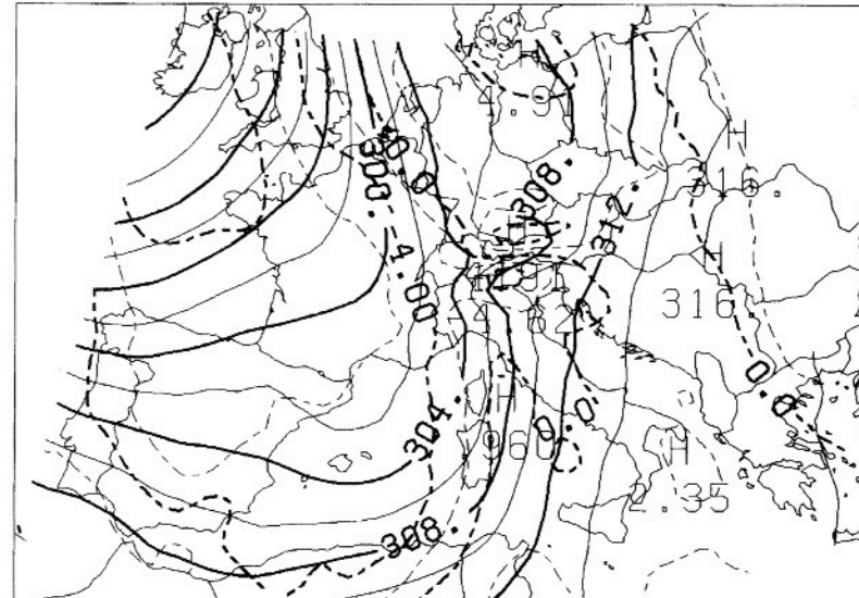
GRIB ANALYSIS AT 06/11/94 00:00 GMT (DOM)
