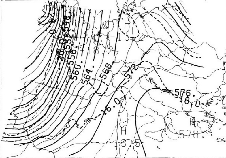
GRIB ANALYSIS AT 04/11/94 00:00 GMT (VEN)
