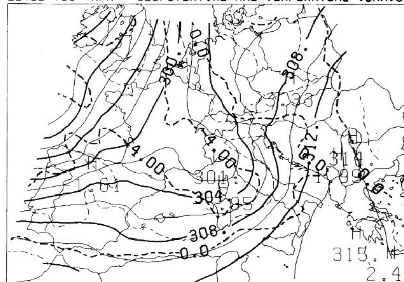
GRIB ANALYSIS AT 06/11/94 12:00 GMT (DOM)
