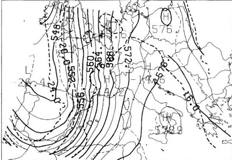
GRIB ANALYSIS AT 05/11/94 00:00 GMT (SAB)
